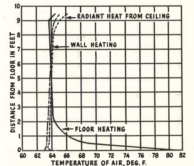
FIG. 5—Comparison of results with radiant heating from ceiling as compared with wall and floor radiant heating.
