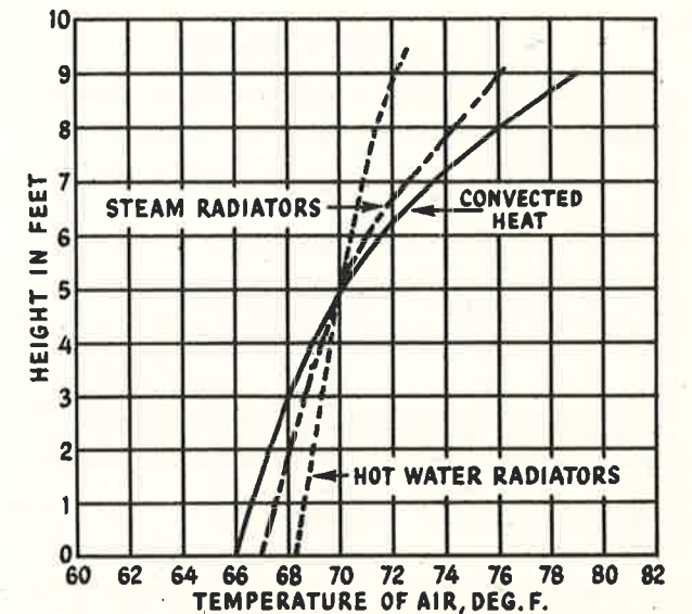
FIG. 4—Average reported temperatures at various heights for heating with radiators and convectors.
